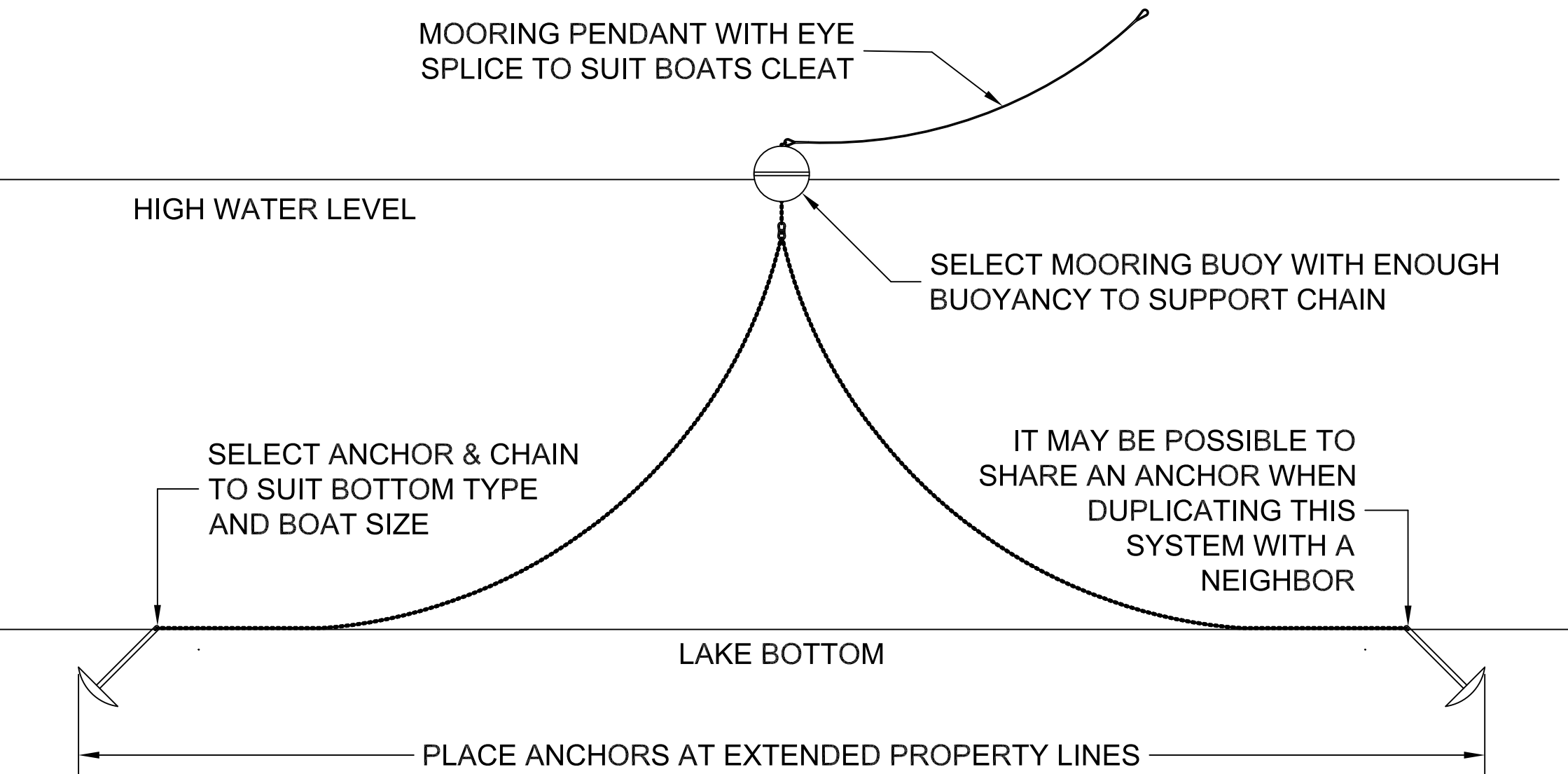
LIMITED SWING MOORING ARRANGEMENT
